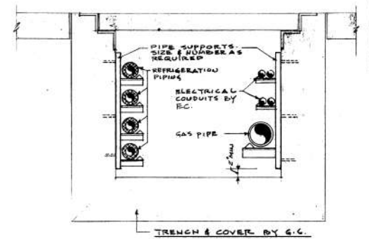
2 PIPE TRENCH DETAIL NO SCALE
